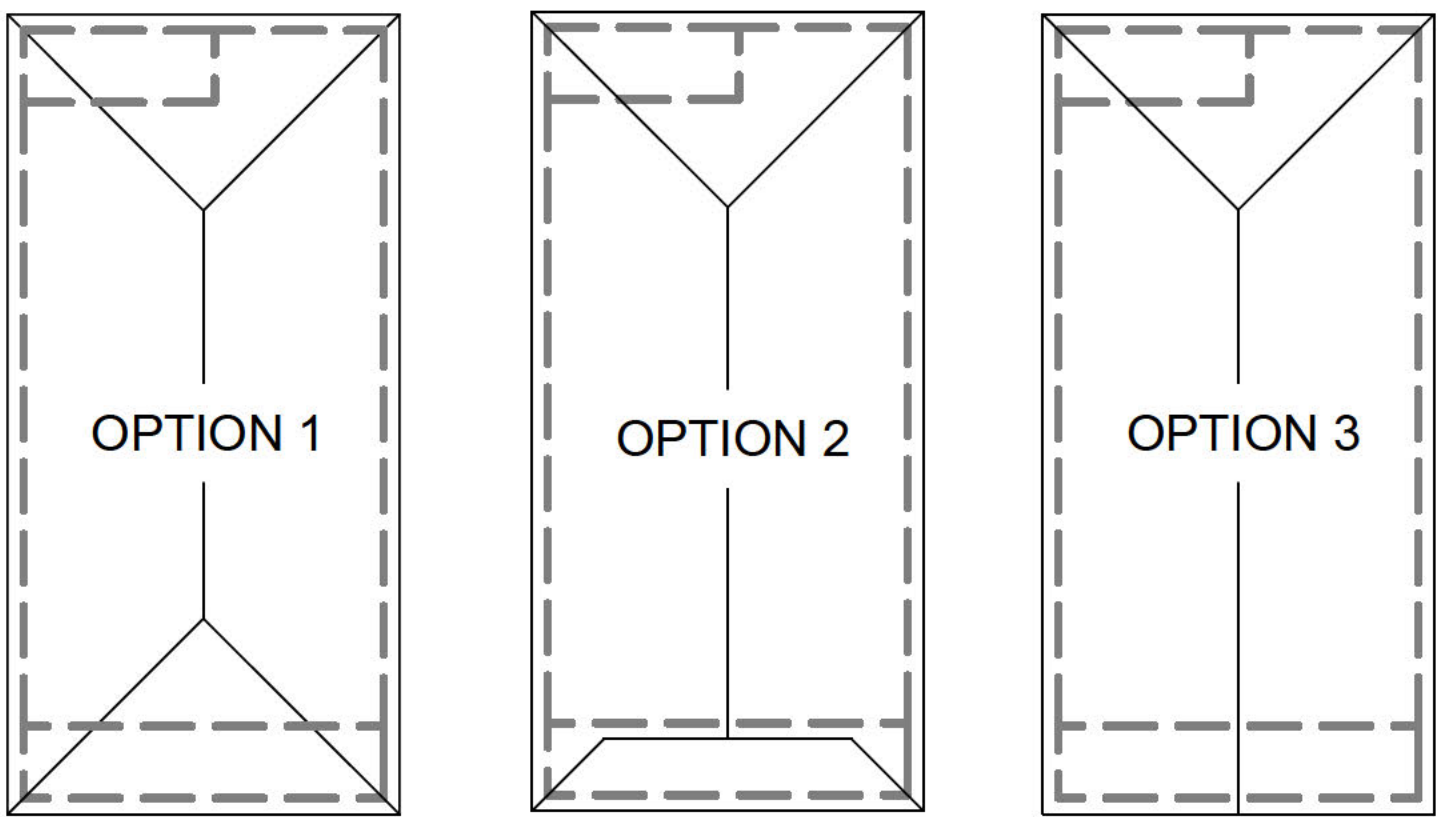
ROOF PLAN
