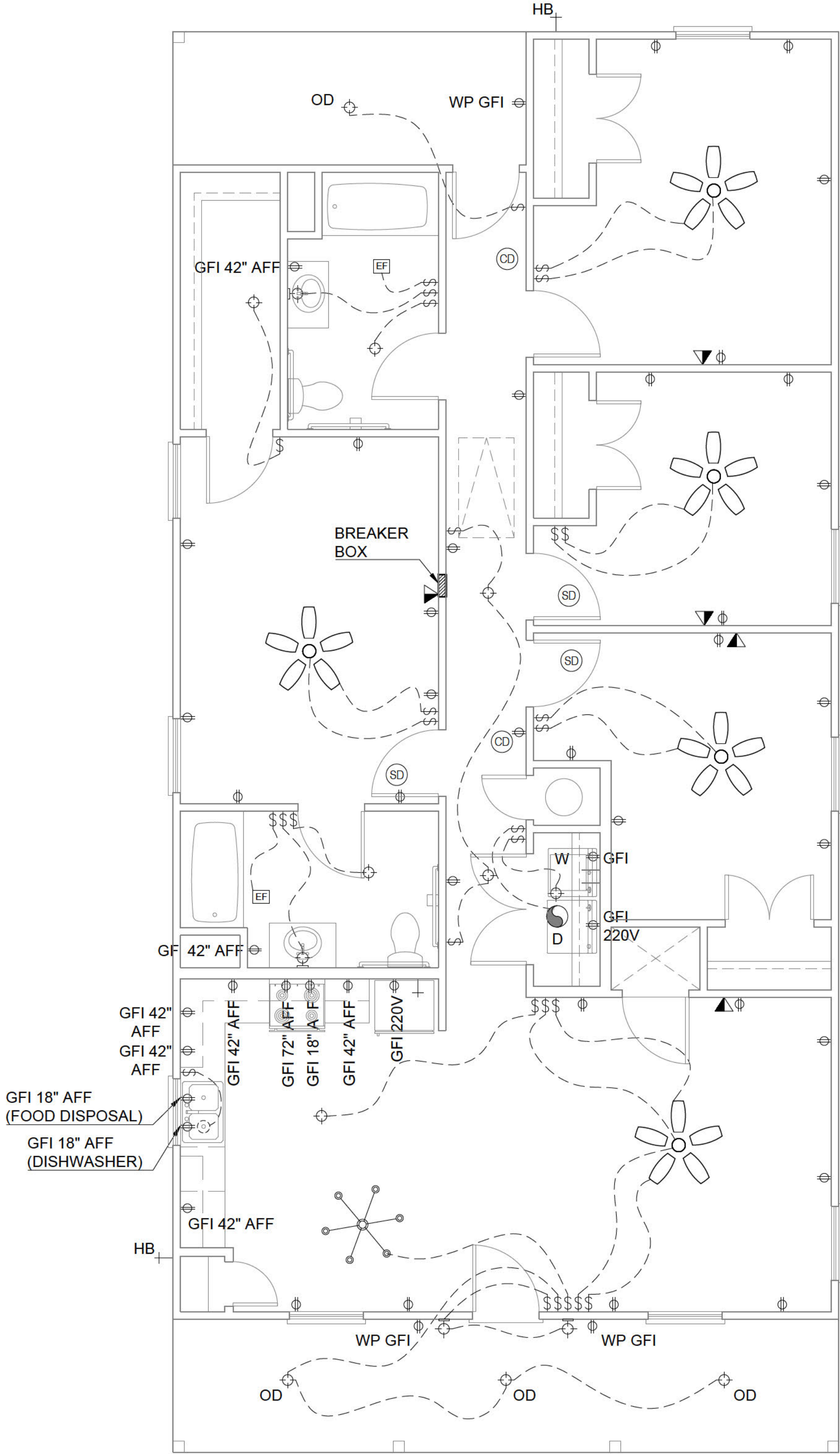
ELECTRICAL PLAN
