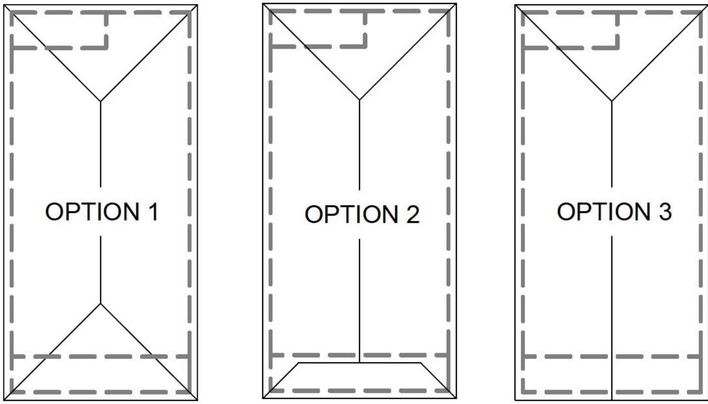
ROOF PLAN
