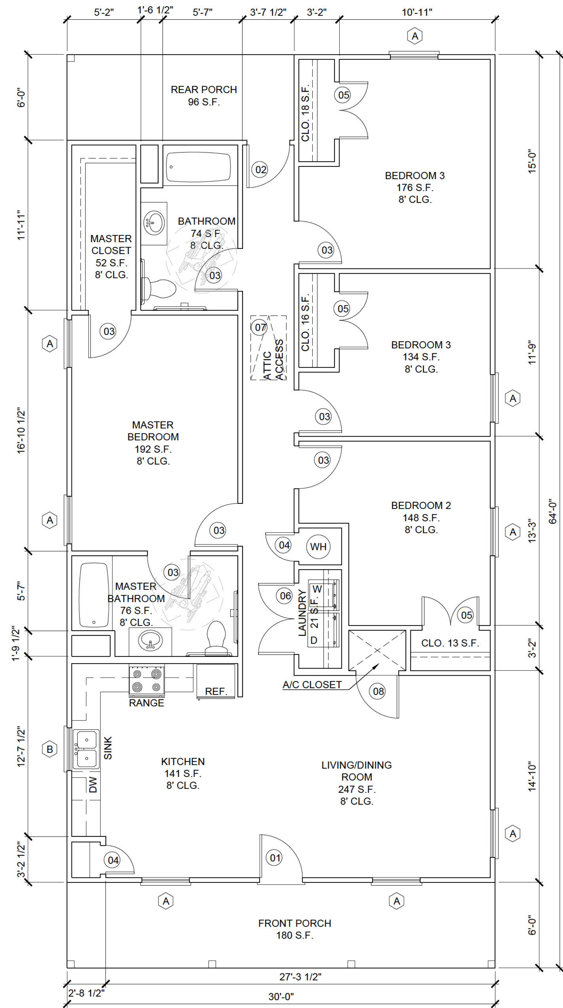
FLOOR PLAN
