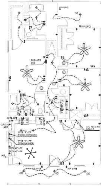
ELECTRICAL PLAN
