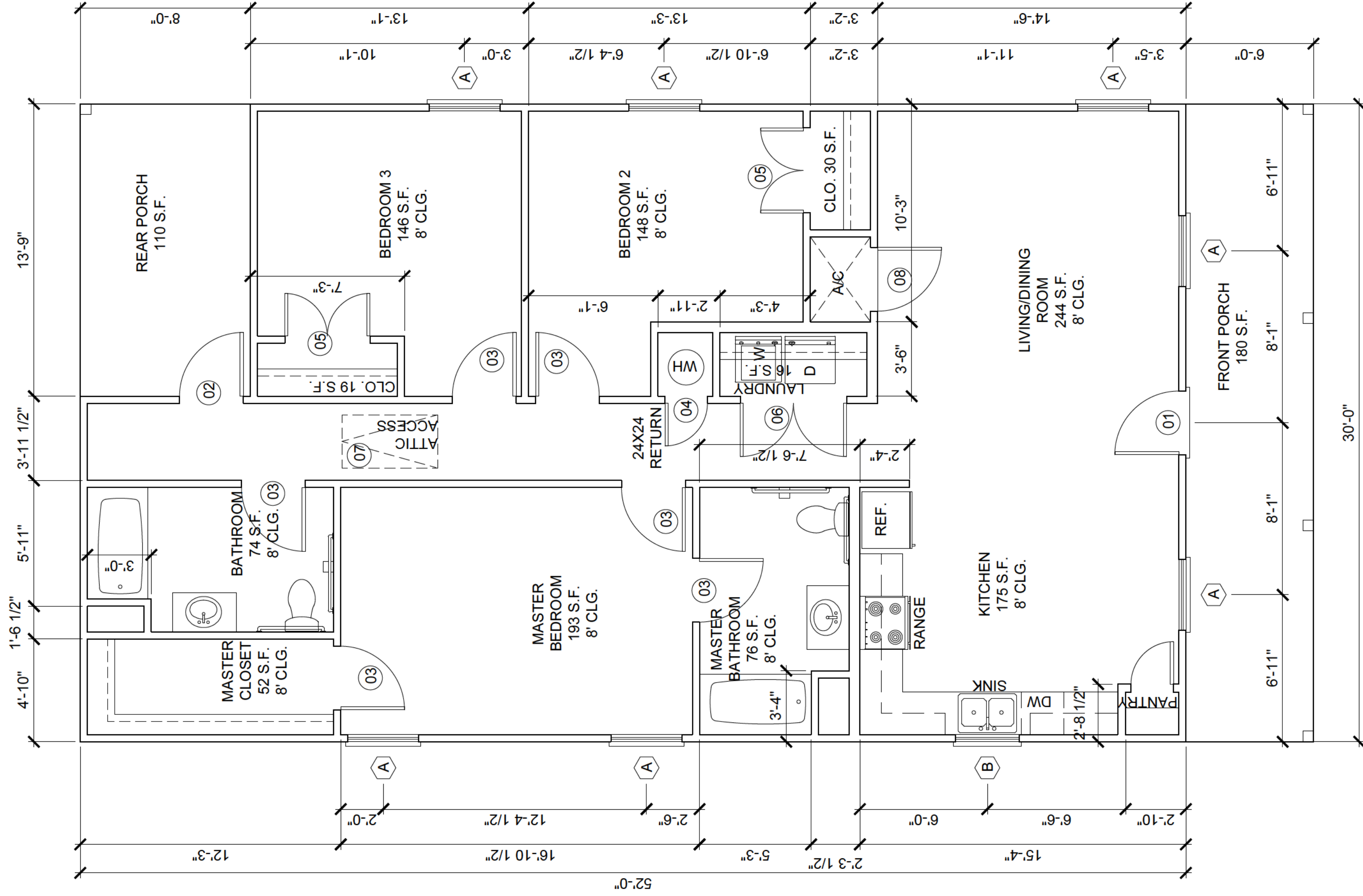
FLOOR PLAN
