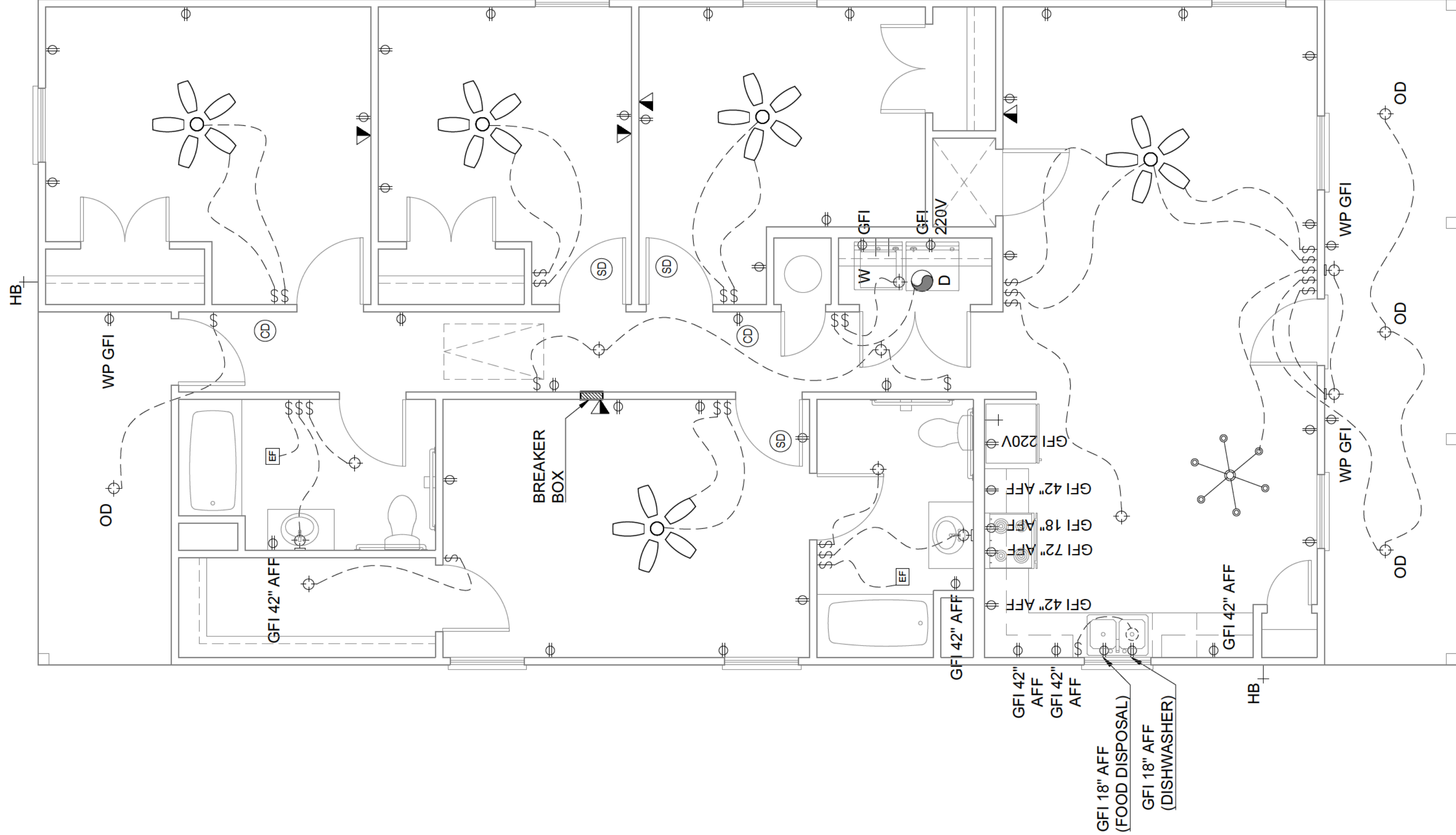
ELECTRICAL PLAN
