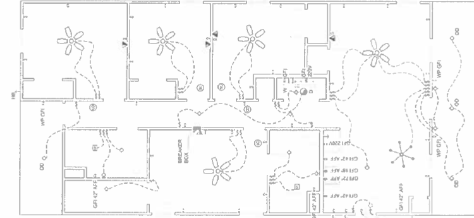
ELECTRICAL PLAN
