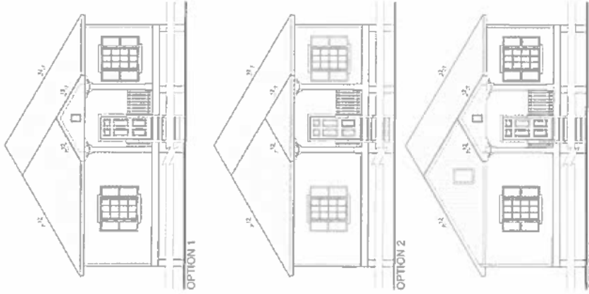
FRONT ELEVATIONS (SIDING)
