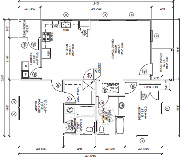
FLOOR PLAN
