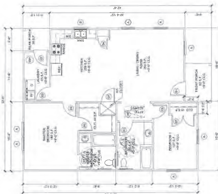
FLOOR PLAN
