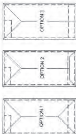
ROOF PLAN
