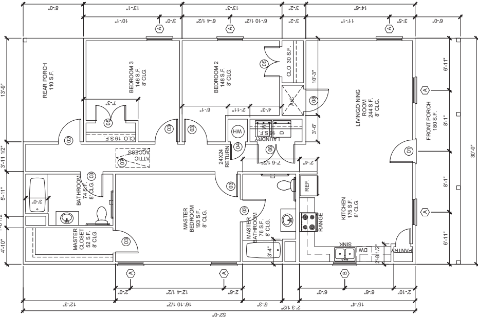
FLOOR PLAN
