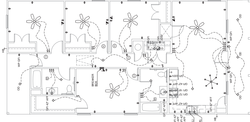
ELECTRICAL PLAN
