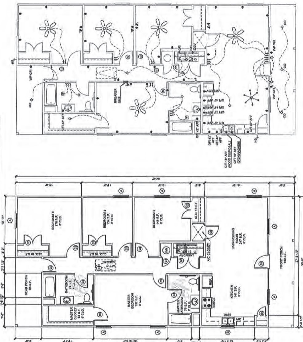
ELECTRICAL PLAN
