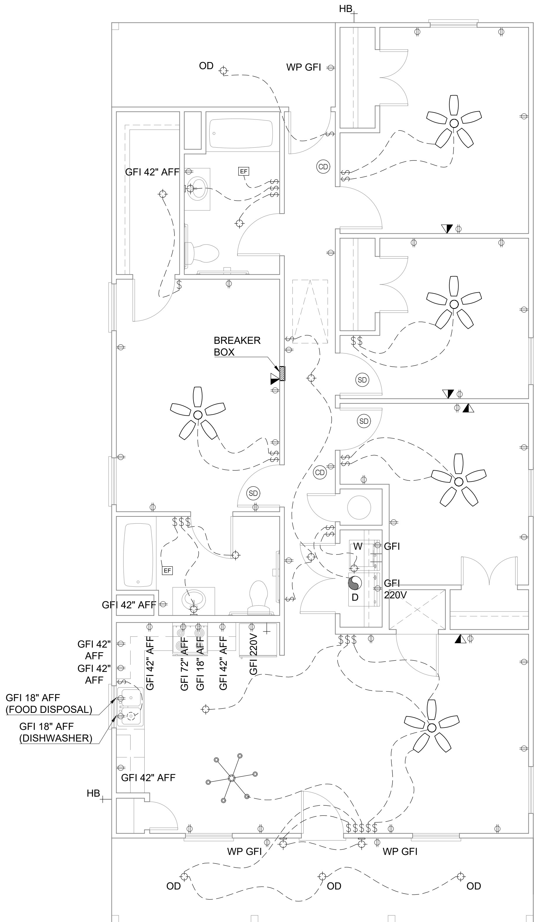
ELECTRICAL PLAN
