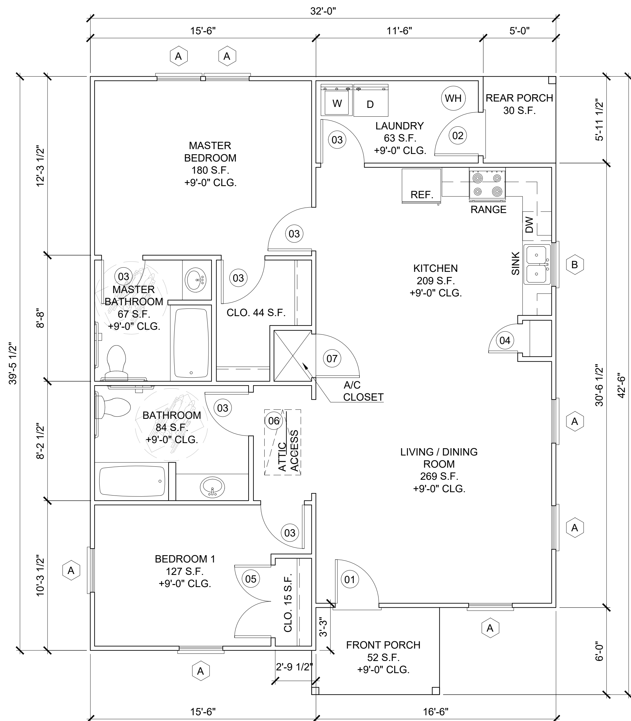
FLOOR PLAN
